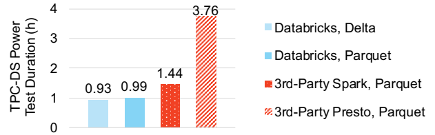
Figure 6: TPC-DS power test duration for Spark on Databricks and Spark and Presto on a third-party cloud service.
